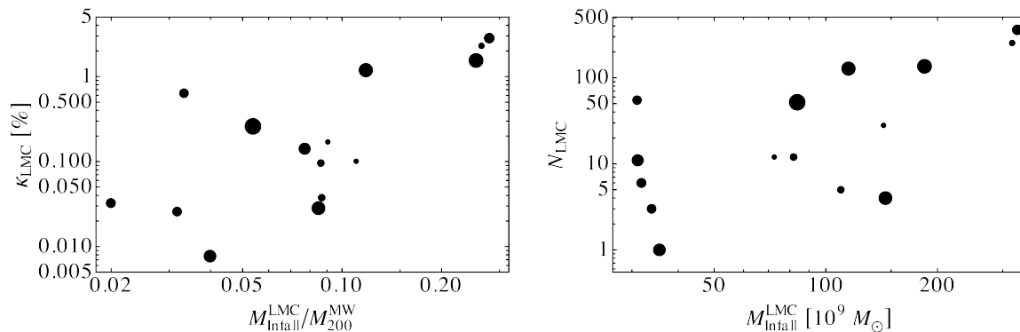
Figure 3. The correlation between \kappa_{\text{LMC}} and M_{\text{Infall}}^{\text{LMC}}/M_{200}^{\text{MW}} (left), and N_{\text{LMC}} and M_{\text{Infall}}^{\text{LMC}} (right) for the 15 MW-LMC analogues. \kappa_{\text{LMC}} and N_{\text{LMC}} are given in the Solar region for the best fit Sun’s position at the simulation snapshot closest to the LMC’s pericenter approach. The sizes of points increase with the distance of the LMC analogues from host at pericenter.
